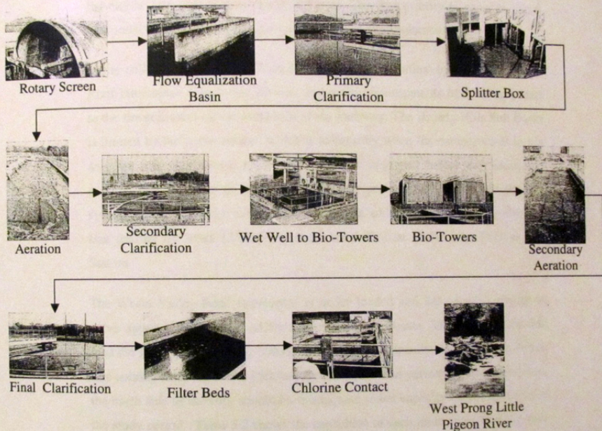
Figure 3.3 Pigeon Forge Wastewater Treatment Plant
