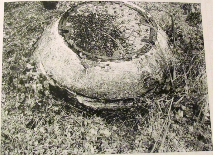
Broken Bell in City Park Sub Basin, Located through USFOS I/I Reduction Efforts
